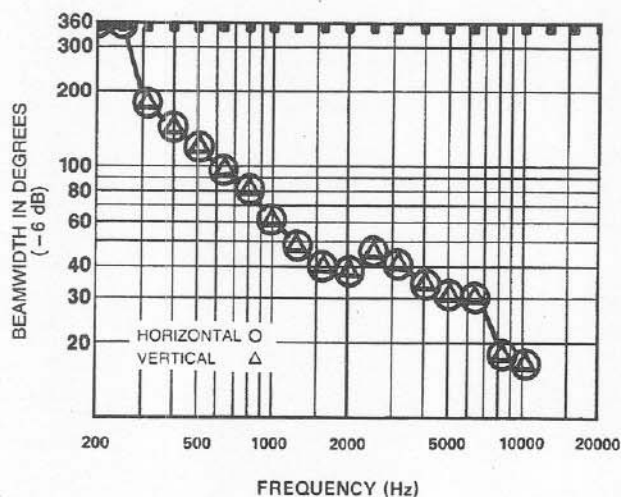
FIGURE 2 PH Beamwidth vs. Frequency
